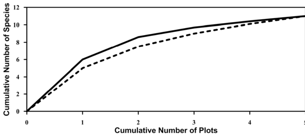
Figure 7. Plotless Species accumulation
