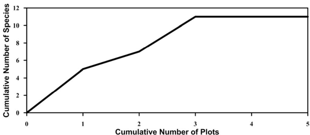
Figure 2. Plotwise species accumulation
