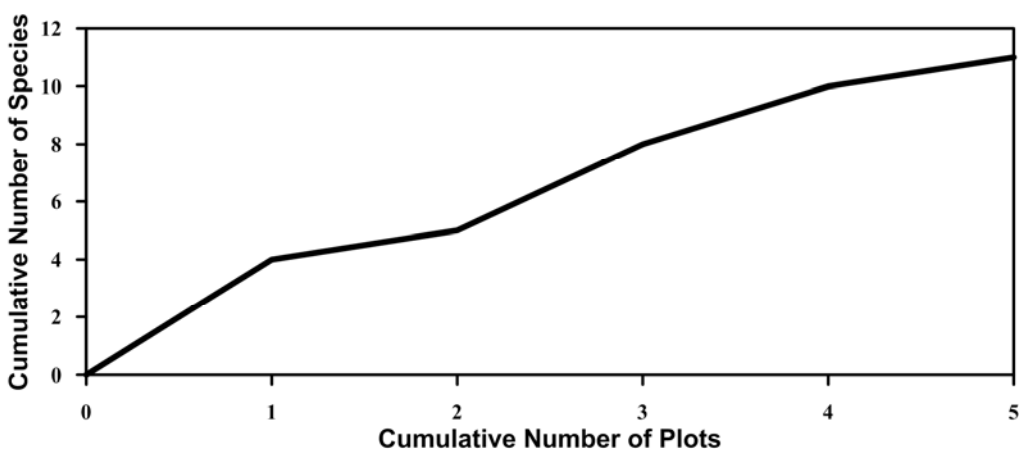
Figure 3. Plotwise species accumulation by different plot order
