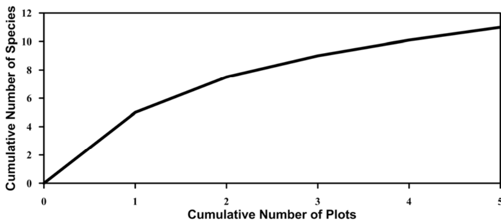
Figure 4. Empirical mean species accumulation
