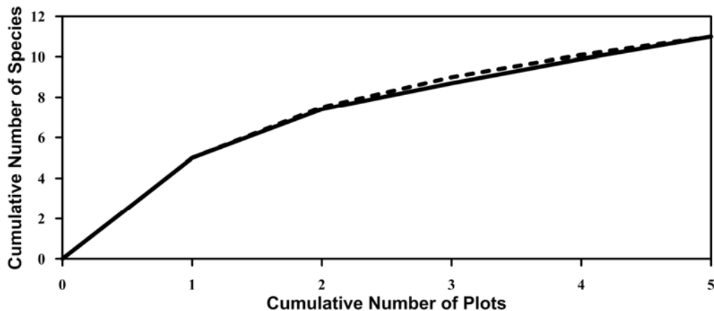
Figure 5. Empirical (solid line) vs. expected (dashed line) mean species accumulation for homogeneously distributed species.
